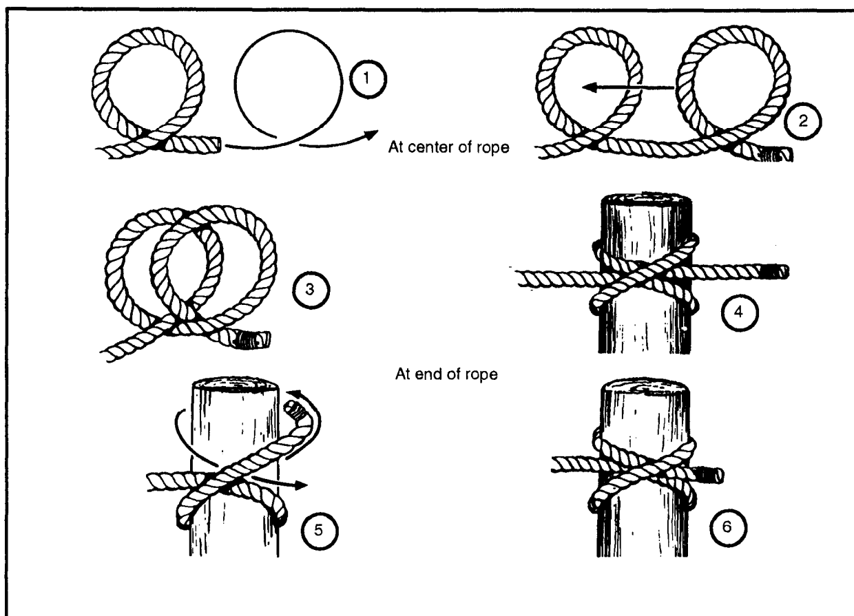
Figure 2-26. Clove hitch
