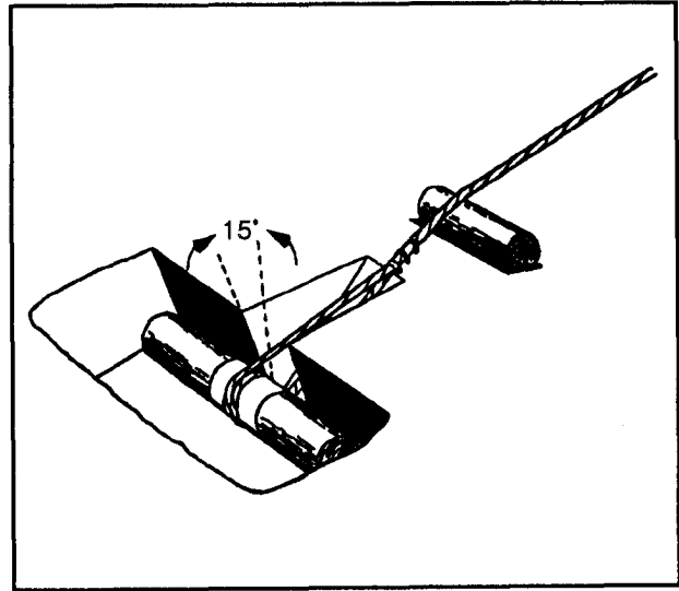
Figure 4-13. Log deadman
