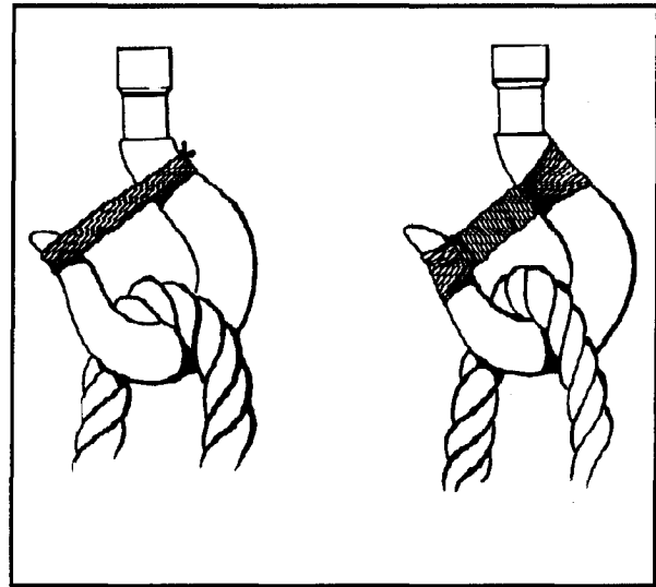
Figure 3-4. Mousing hooks
